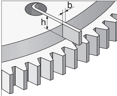
ZAN / ZFN = Reference mark – flag
