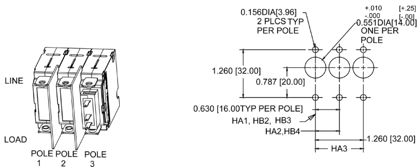
MULTI-POLE IDENTIFICATION SCHEME AS VIEWED FROM TERMINAL END OF BREAKER.
